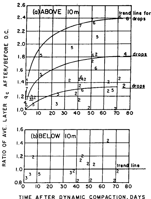
FIGURE 7 - EFFECTS OF TIME, NO. OF DC DROPS, AND DEPTH OF SOIL ON THE RELATIVE IMPROVEMENT IN LAYER AVE. q_c FROM CPTs (Nos. denote drops/data pt.)
